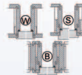
Holzfutter/ Blockzarge
