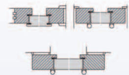
Stockzarge/ Blendrahmen
